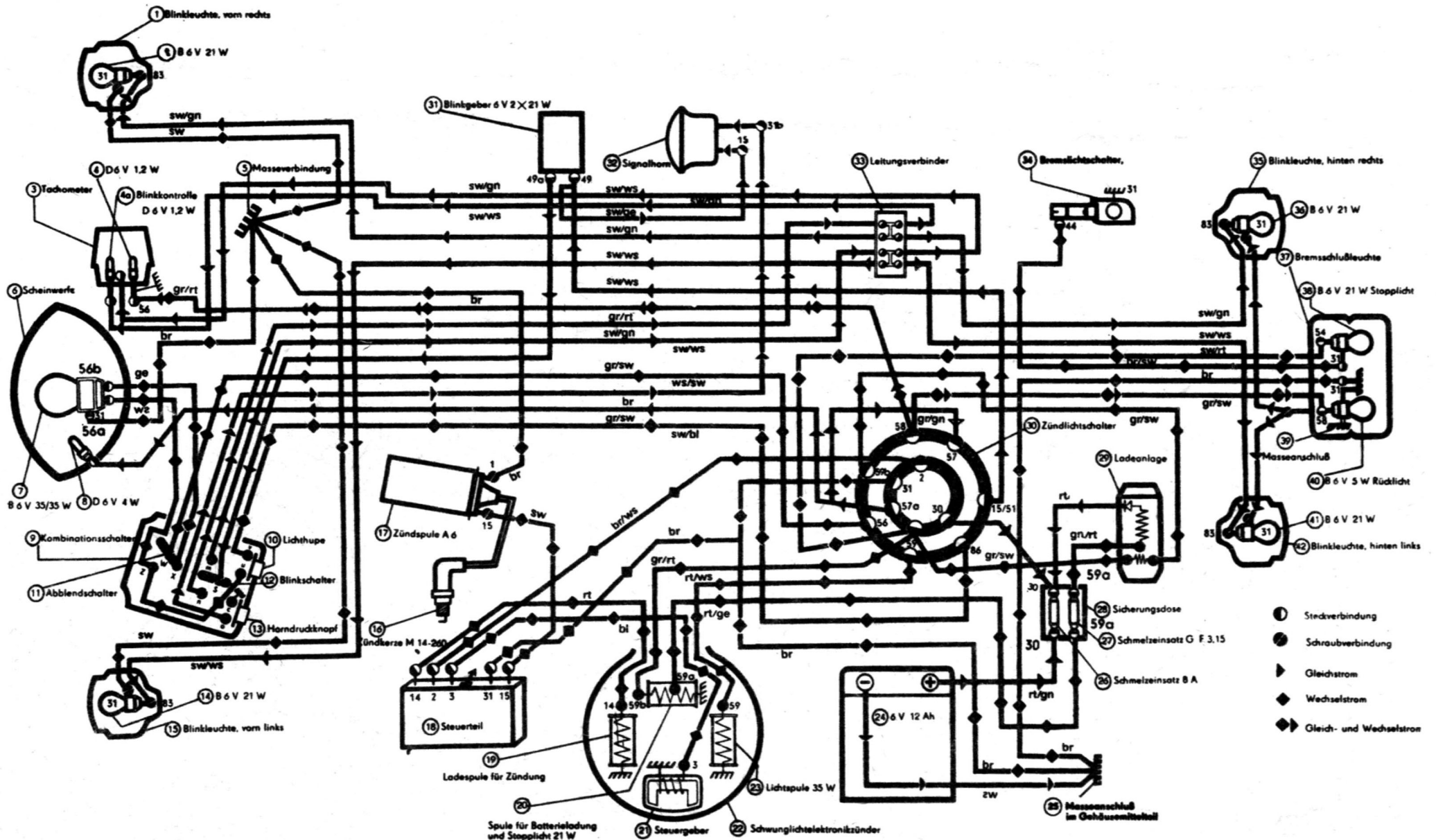
Schaltplan S51 B2-1, S51 B3-1, S51 B4-1
